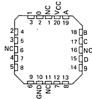
SN54LS445 . . . FK PACKAGE SN74LS445 . . . FN PACKAGE (TOP VIEW)
