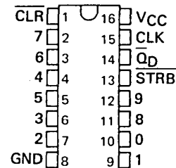
SN74142 . . . J OR N PACKAGE (TOP VIEW)
