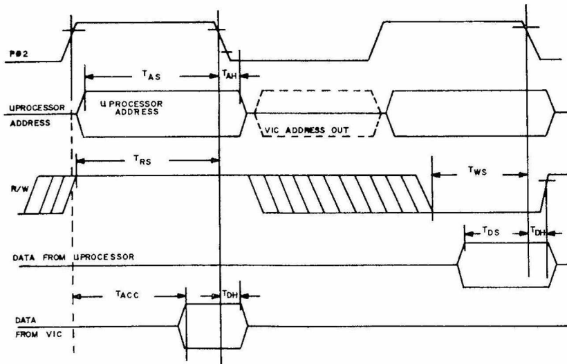
MICROPROCESSOR READ/WRITE TIMING TO VIC
