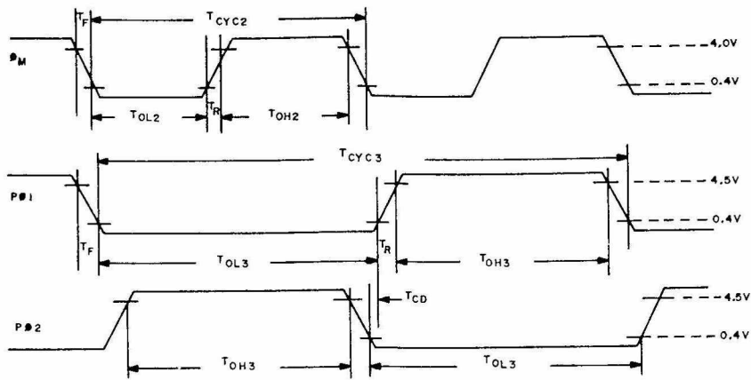
VIC OUTPUT CLOCKS
