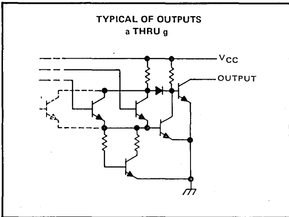
'246, '247
