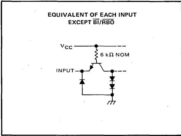
'246, '247
