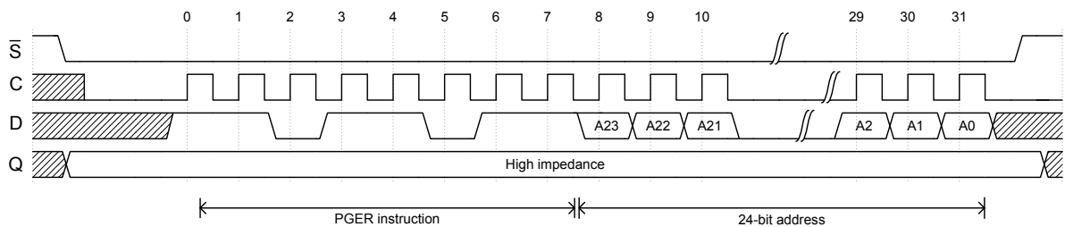
Figure 23. Page erase
