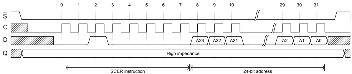
Figure 22. Sector erase
