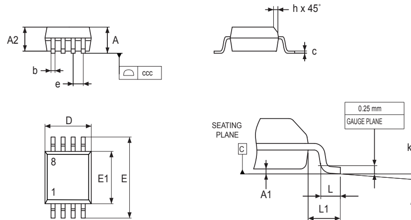
Figure 40. SO8N - Outline
